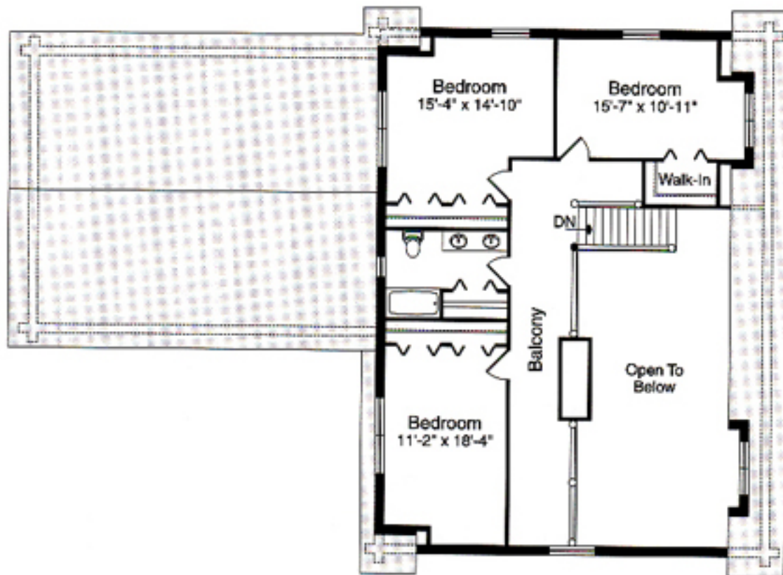
Blue Ridge 2,894 sq. ft.
