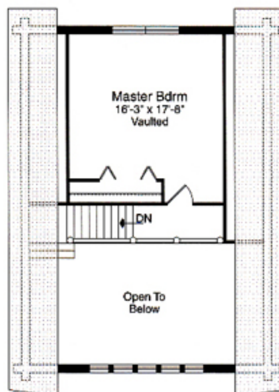
Second Floor 352 sq. ft.
