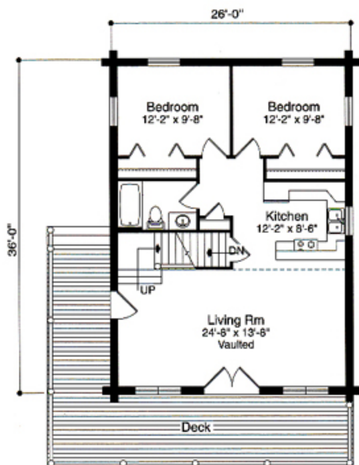
First Floor 936 sq. ft.
