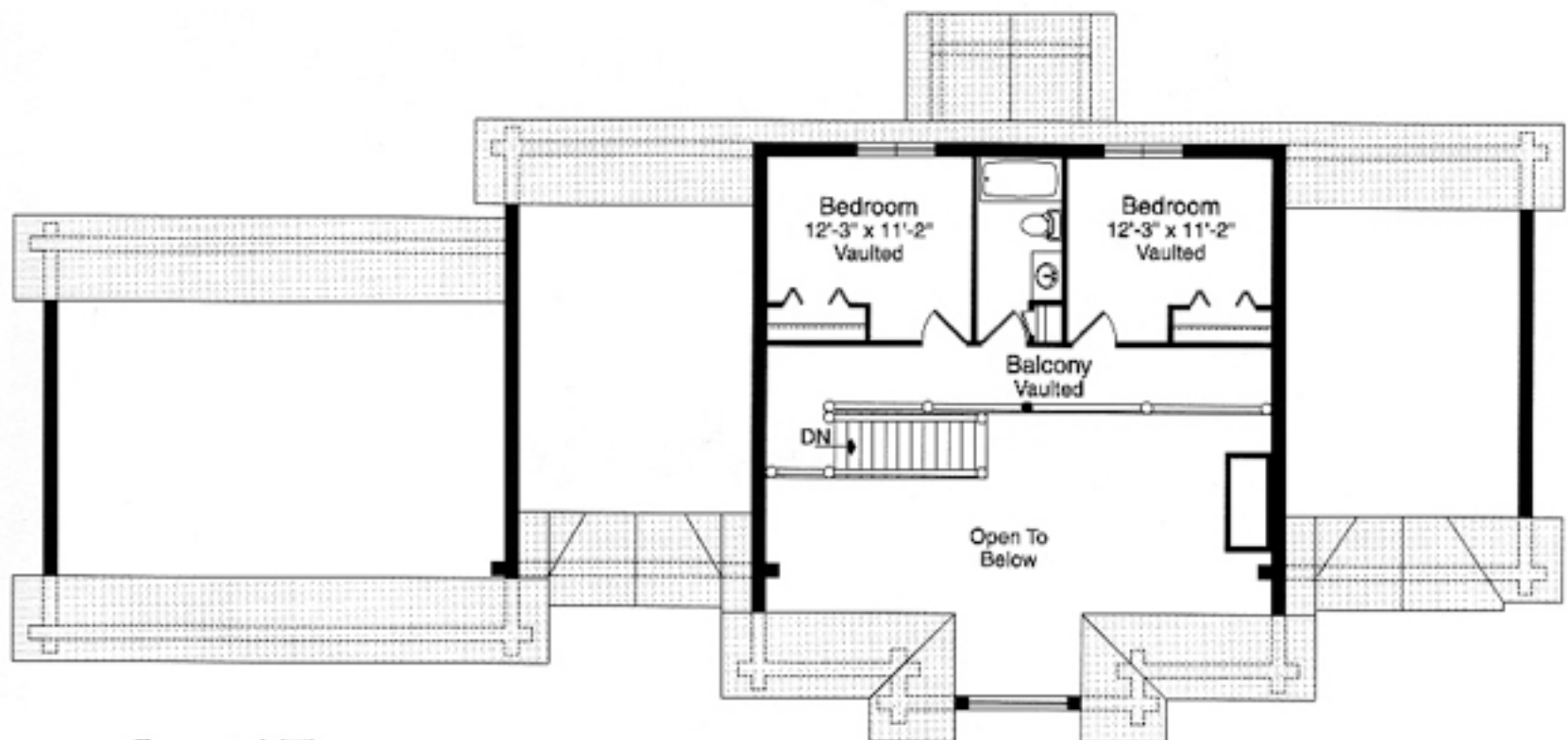
Second Floor 547 sq. ft.
