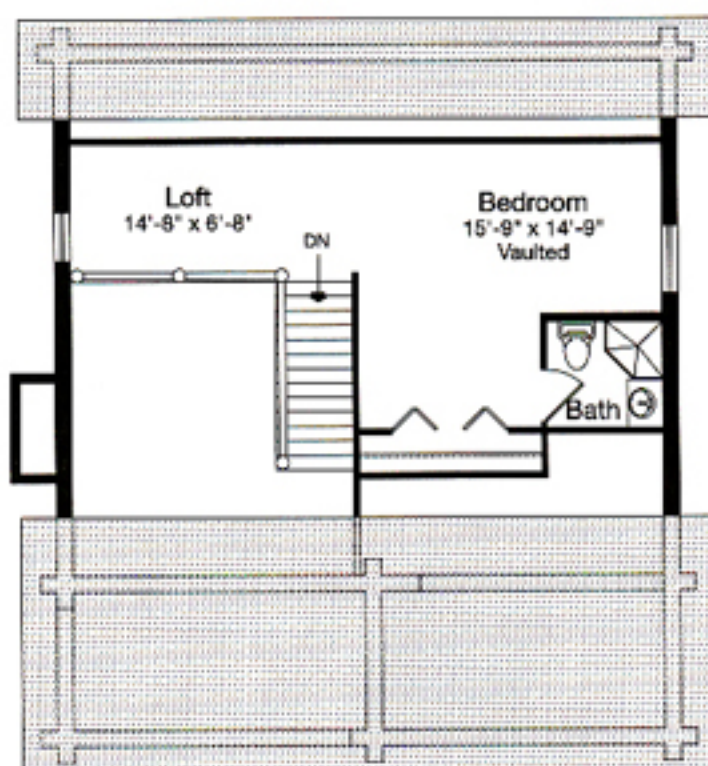
Second Floor 896 sq. ft.
