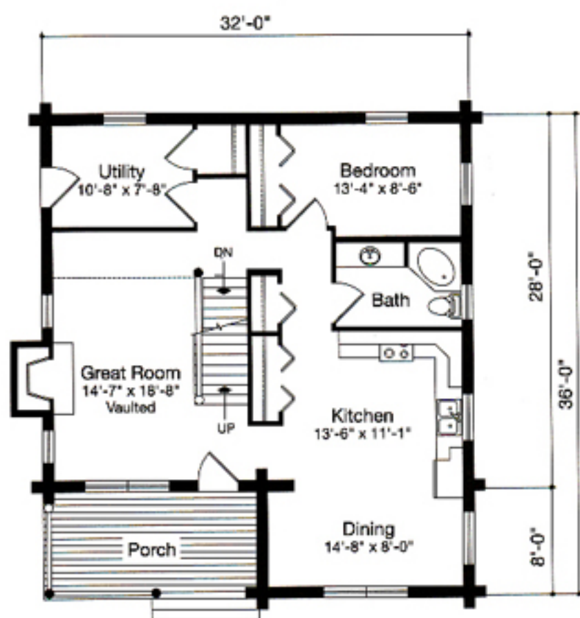
First Floor 1,024 sq. ft.
