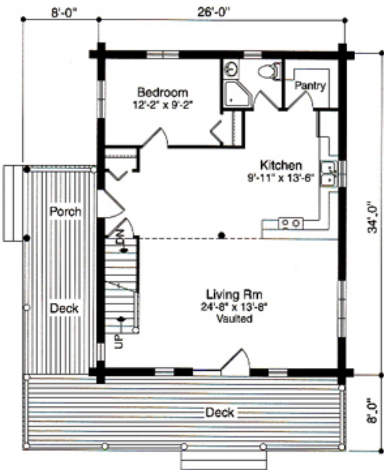
First Floor 884 sq. ft.
