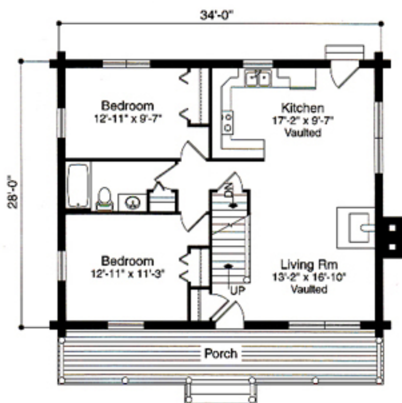
First Floor 952 sq. ft.
