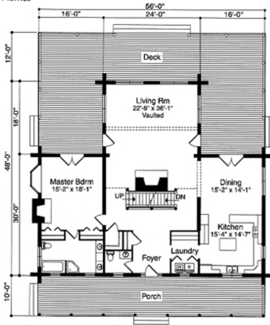
First Floor 2,112 sq. ft.
