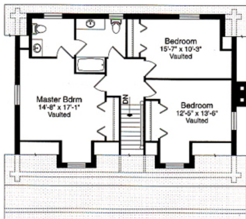
Second Floor 832 sq. ft.
