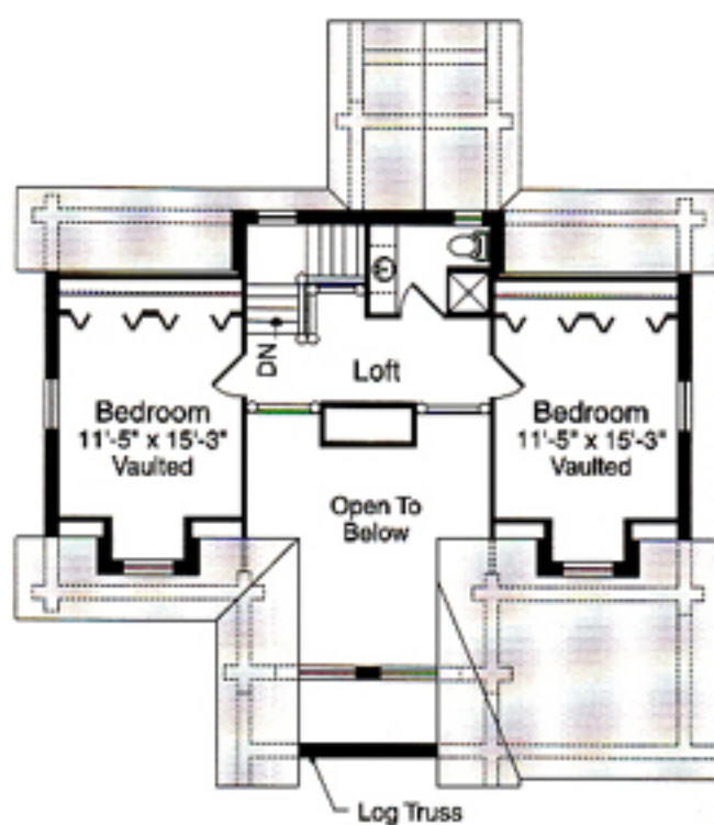
Second Floor 560 sq. ft.
