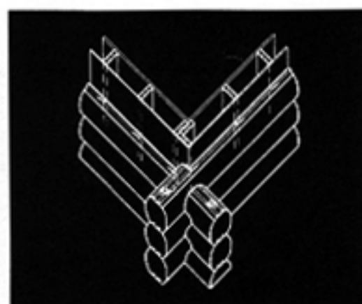
Half Log Tongue & Groove
