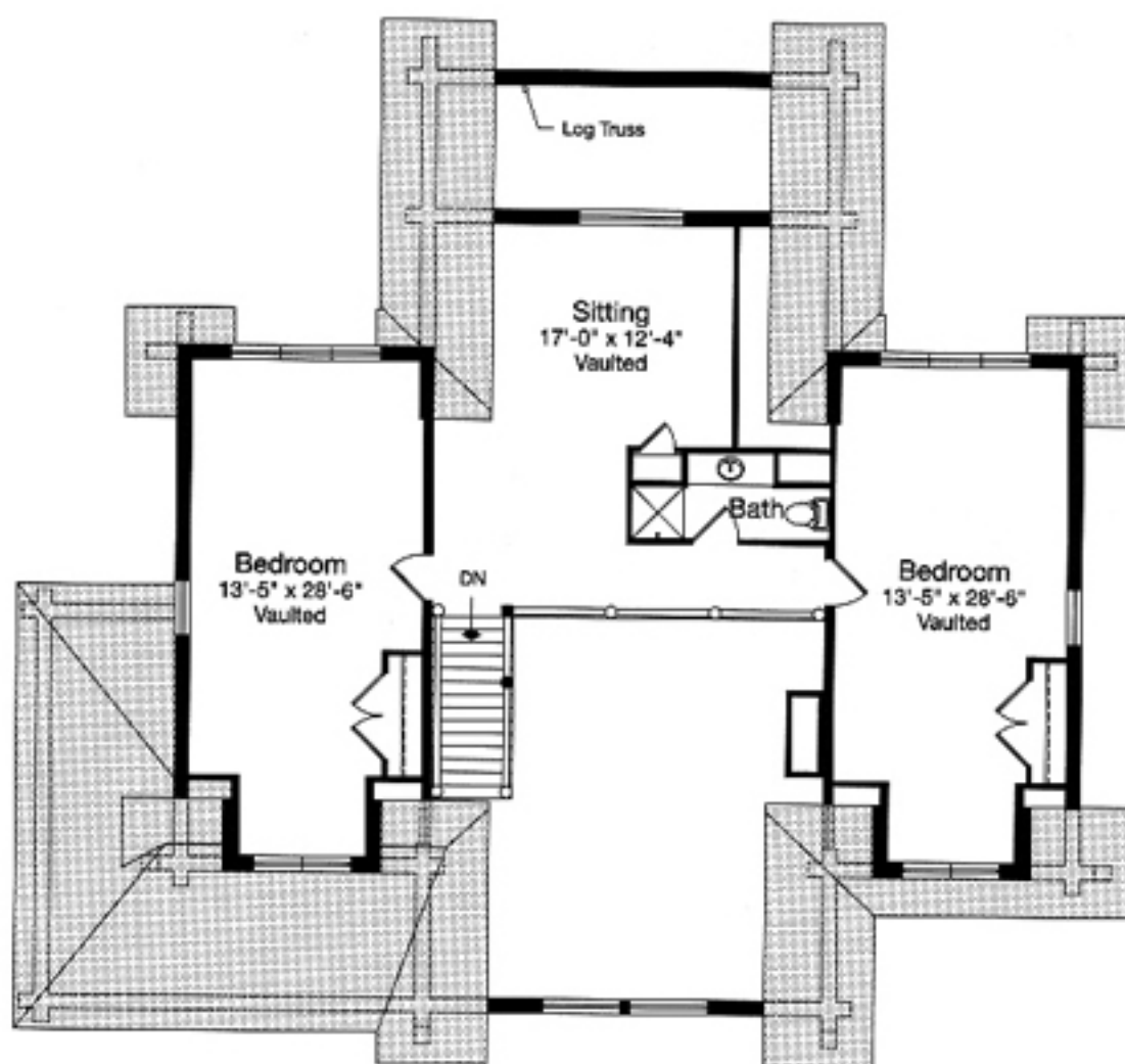
Second Floor 1,107 sq. ft.
