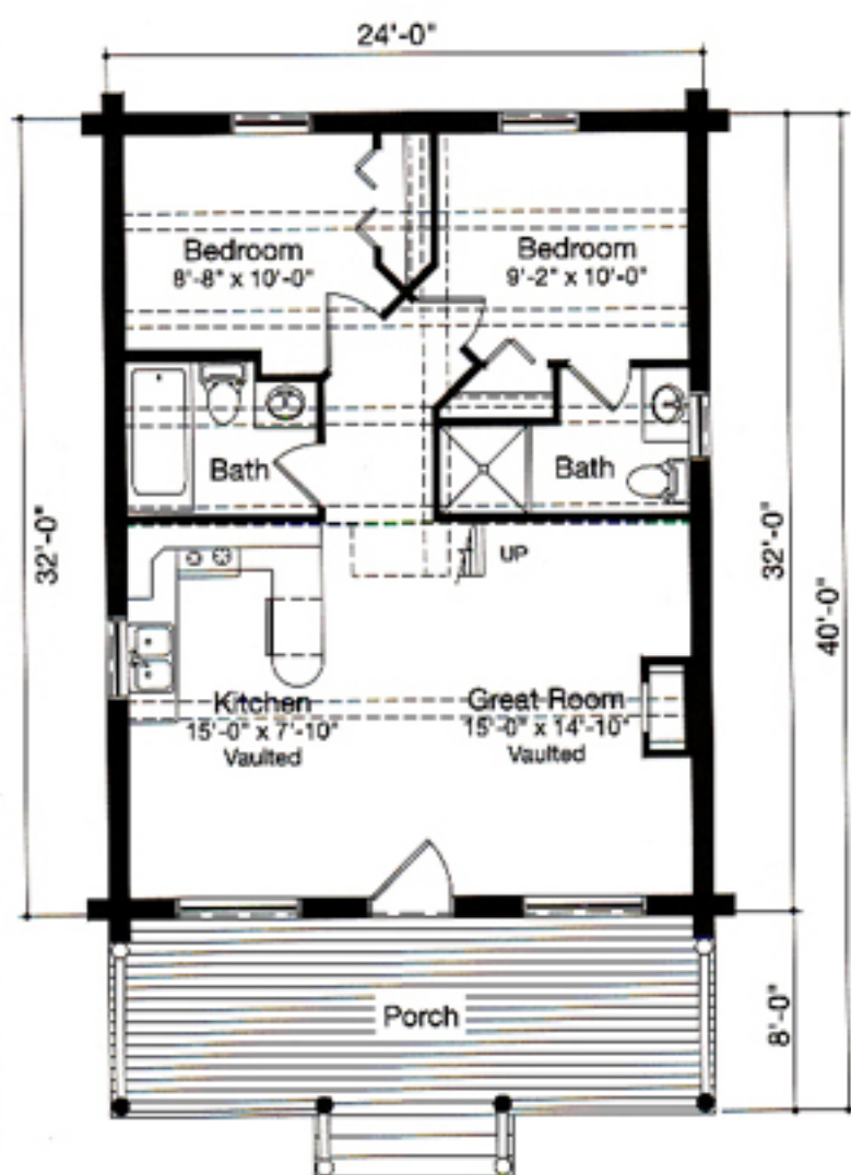
First Floor 768 sq. ft.
