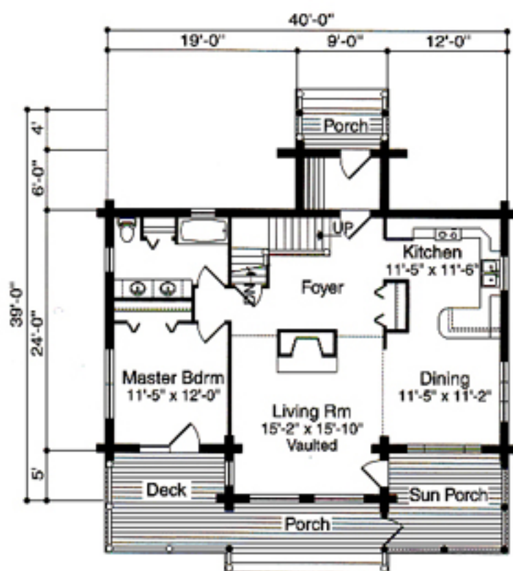
First Floor 1,114 sq. ft.
