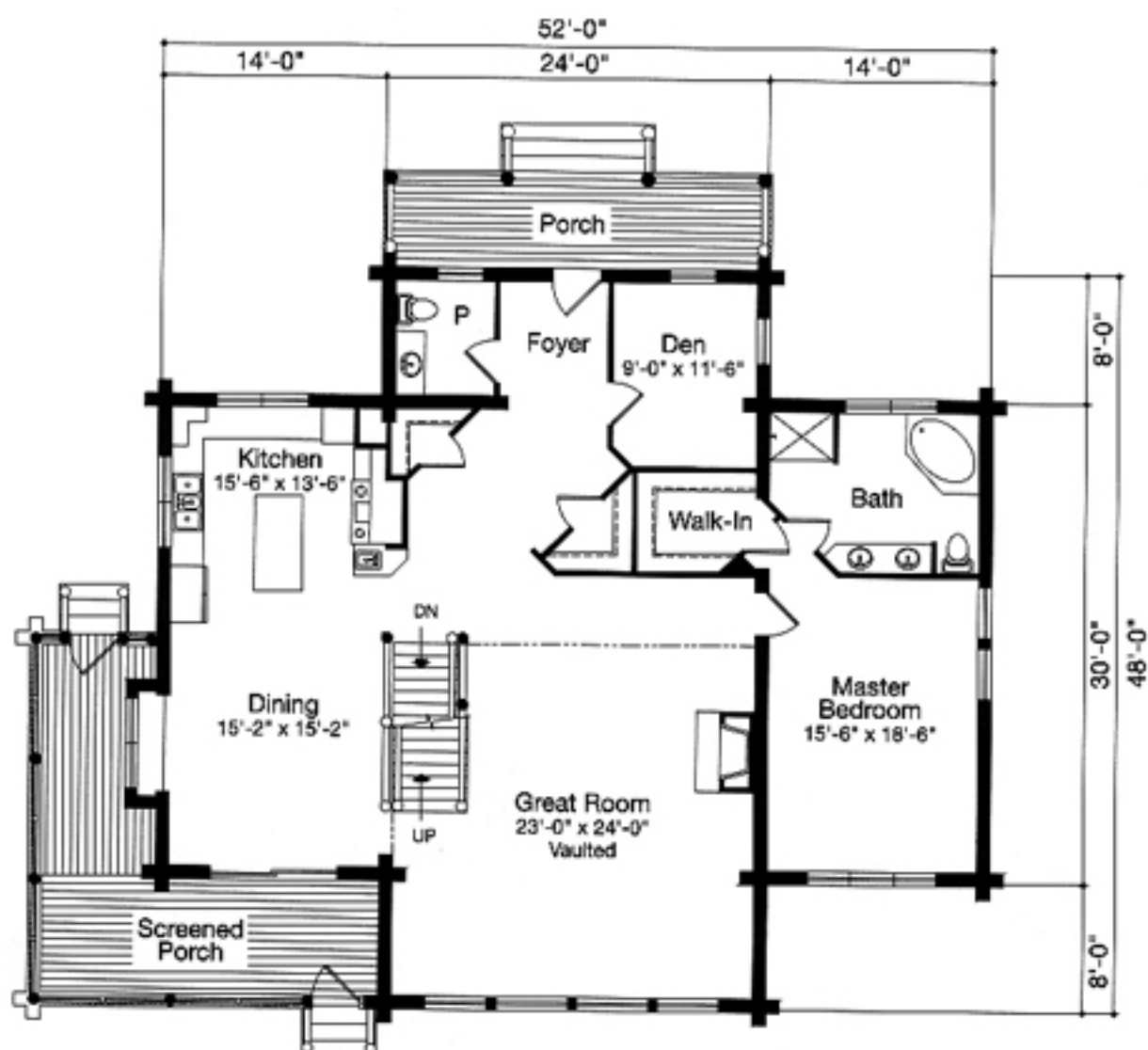
First Floor 2,068 sq. ft.
