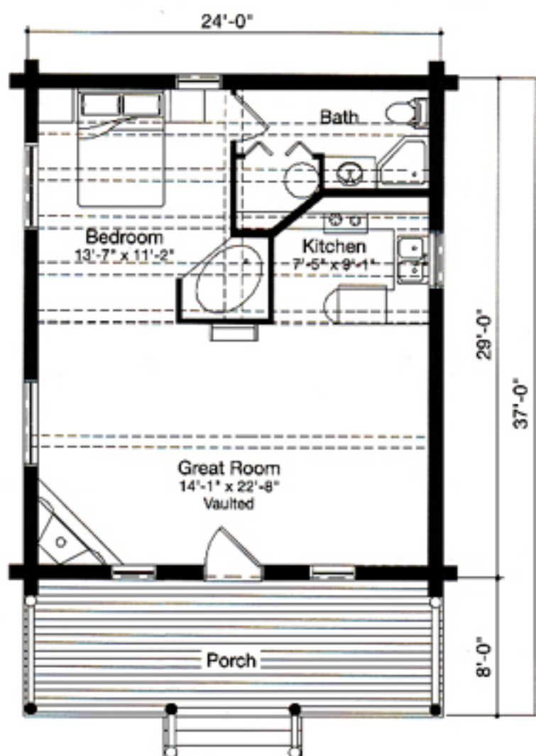
First Floor 696 sq. ft.
