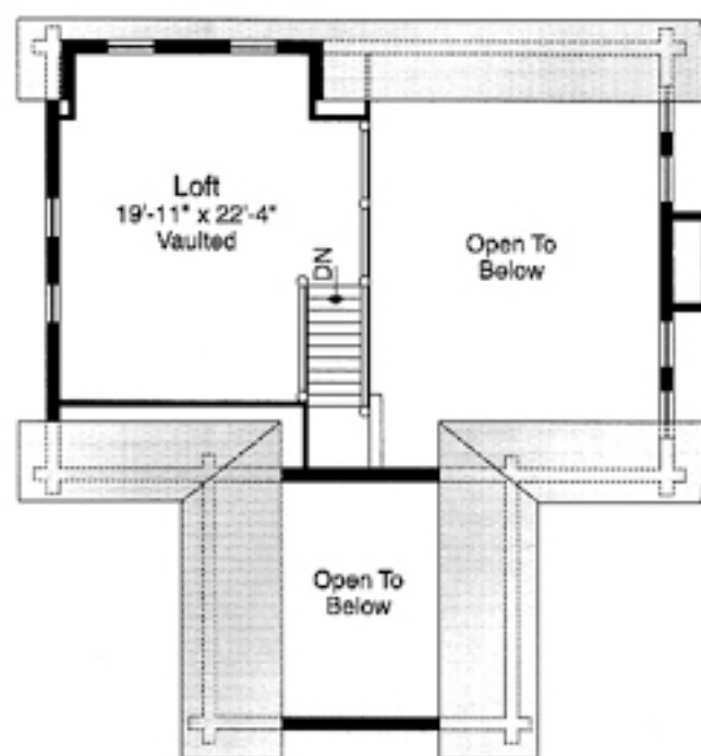
Second Floor 425 sq. ft.
