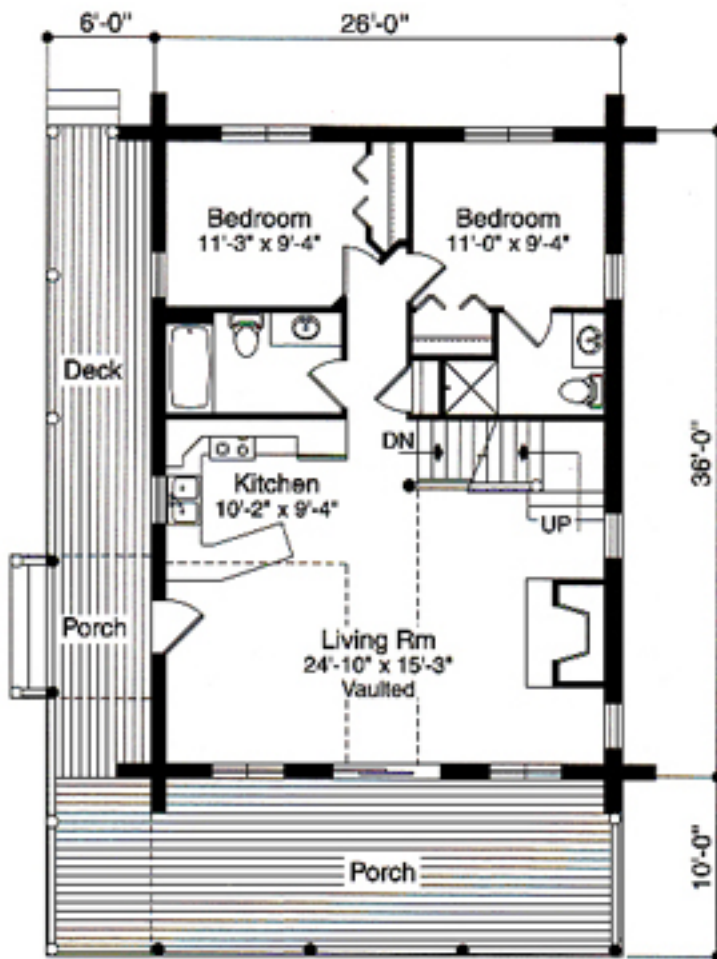
First Floor 936 sq. ft.
