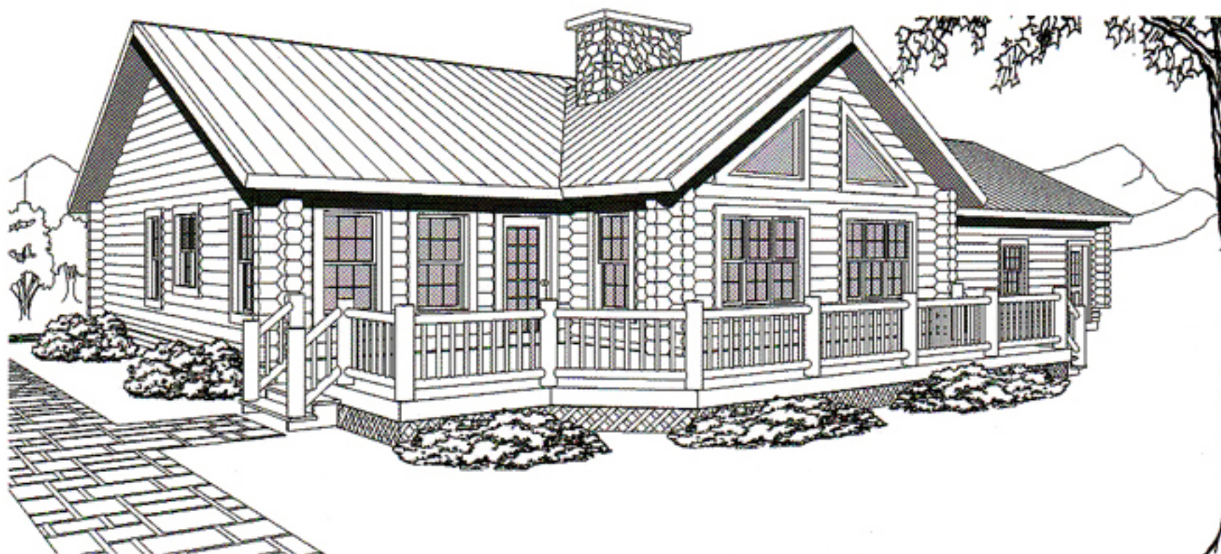
the Dover 1,800 sq. ft.
